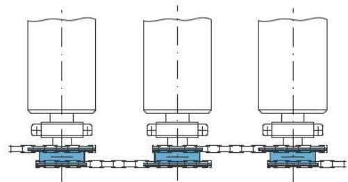
Roller conveyor
